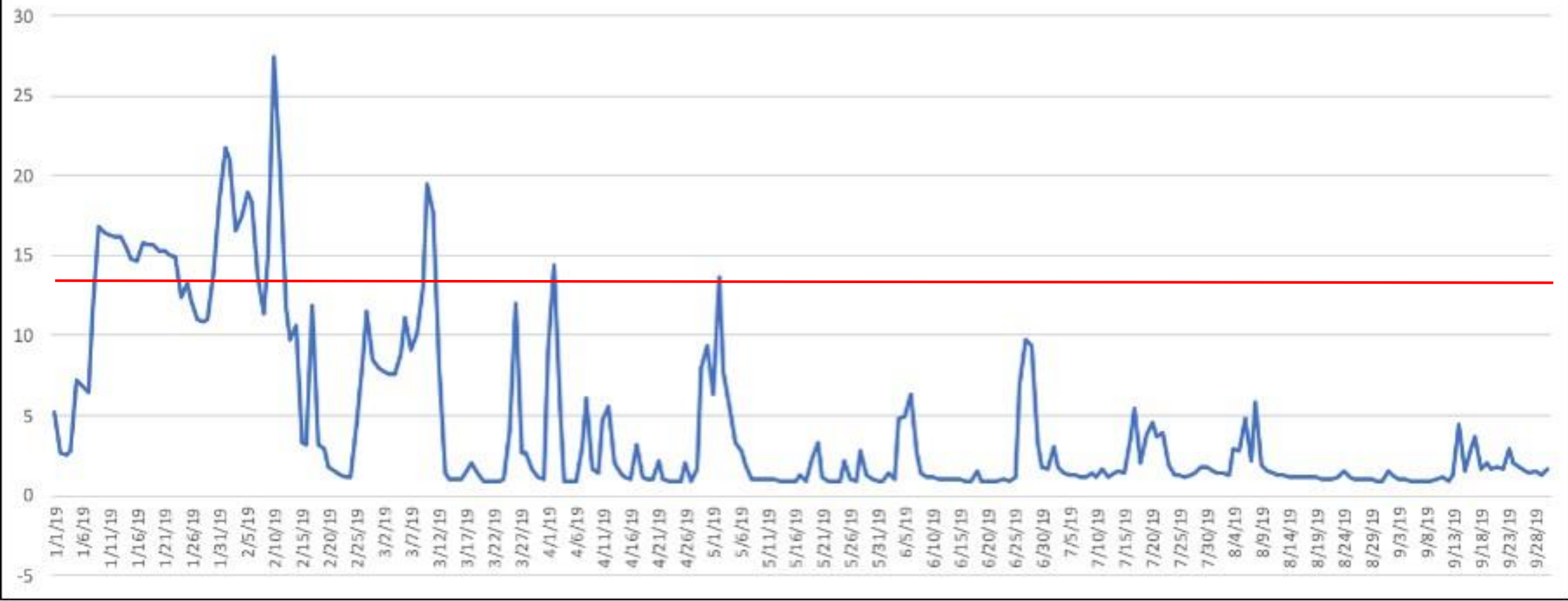
2019 Waikoko Gage - Daily Average Combined Ditch Flow (mgd) (2019 average 2019 to date 4.6 mgd)
